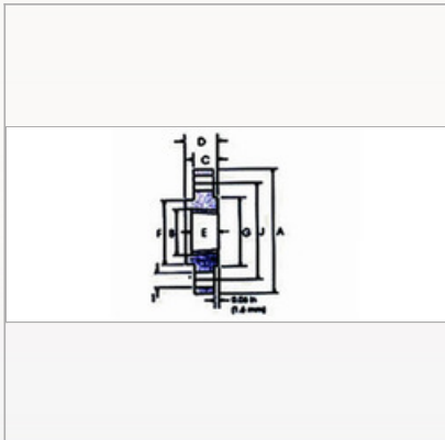
ANSI B 16.5 Class 150 lb
