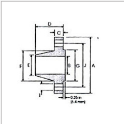
ANSI B 16.5 Class 1500 lb
