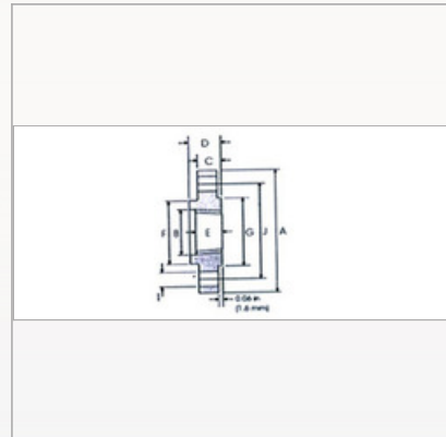
ANSI B 16.5 Class 300 lb
