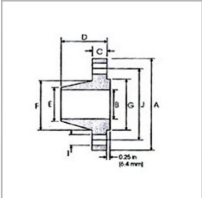
ANSI B 16.5 Class 600 lb Weld Neck Flange
