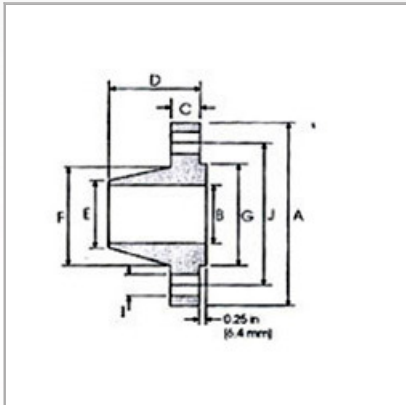
ANSI B 16.5 Class 900 lb Weld Neck Flanges
