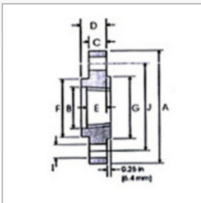
ANSI B 16.5 Class 2500 lb Weld Neck Flanges
